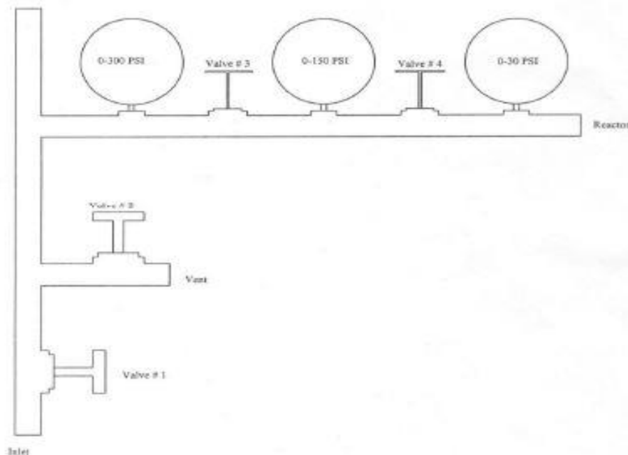
Drawing of Manifold (type “B”)
